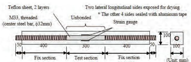
(ii) Restrained cracking test specimen and observed strain
